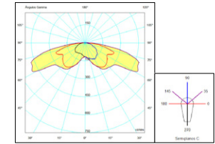
LED 4C
