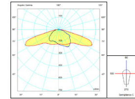
LED 3C
