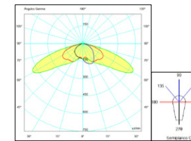
Microreflector 45W-60W
