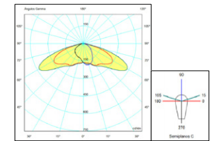
Microreflector 90W-140W
